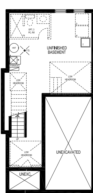
BASEMENT PLAN, EL. '1803-A'
